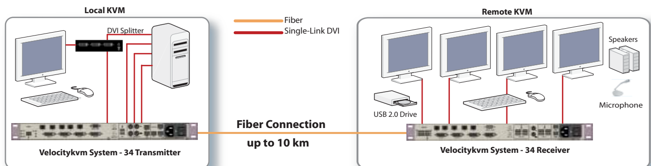
Typical application extending DVI video and peripheral devices using the Velocitykvm System - 34
