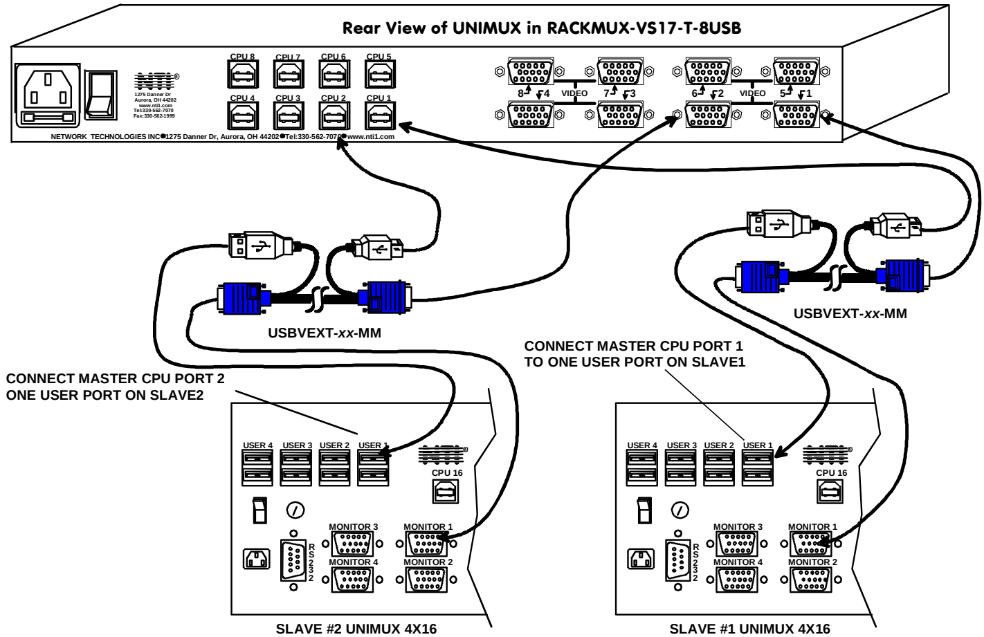
Figure 30- Master to slave cable connections- multi-user switches
