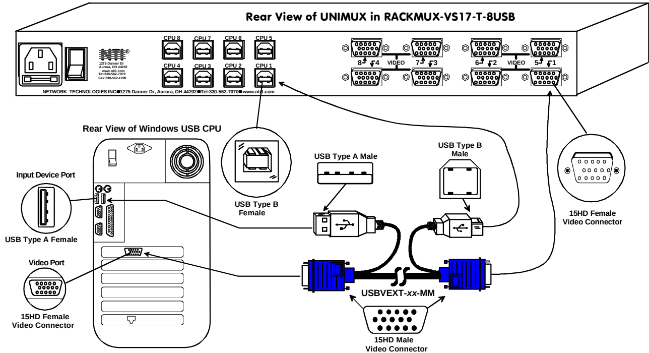
Figure 8- Connect each CPU
