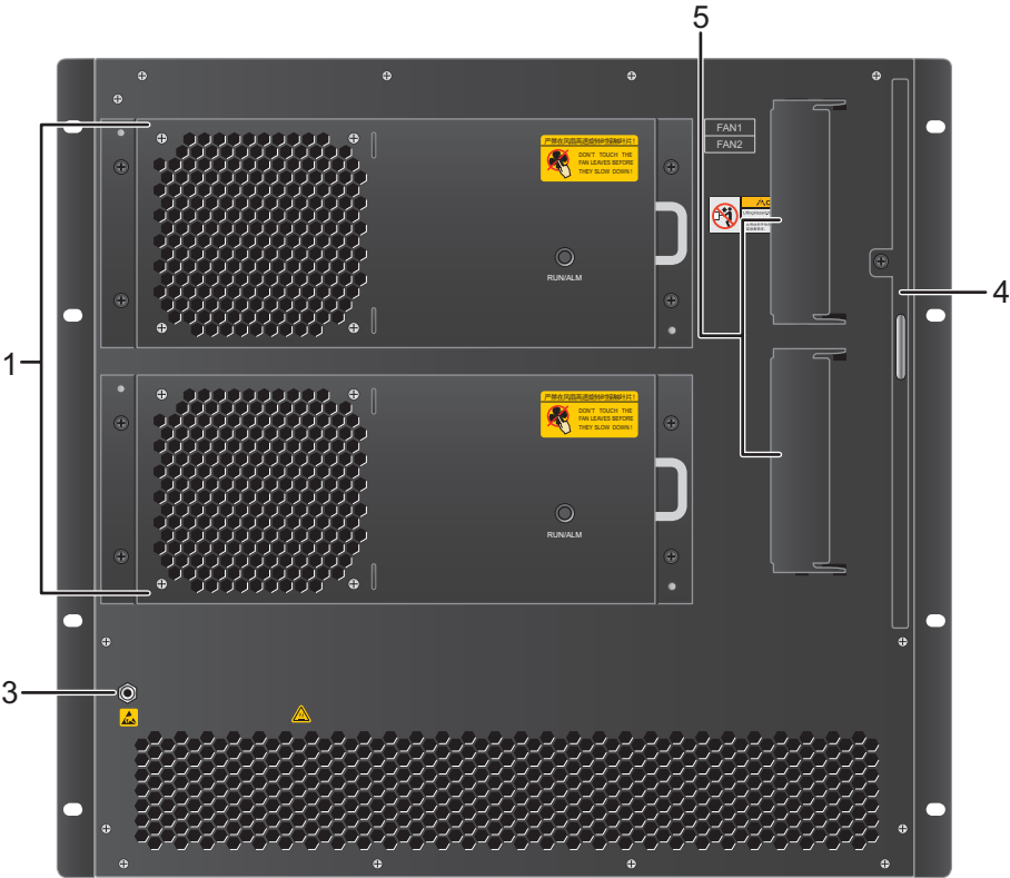
Figure 4-11 S7706 chassis structure (rear view)
