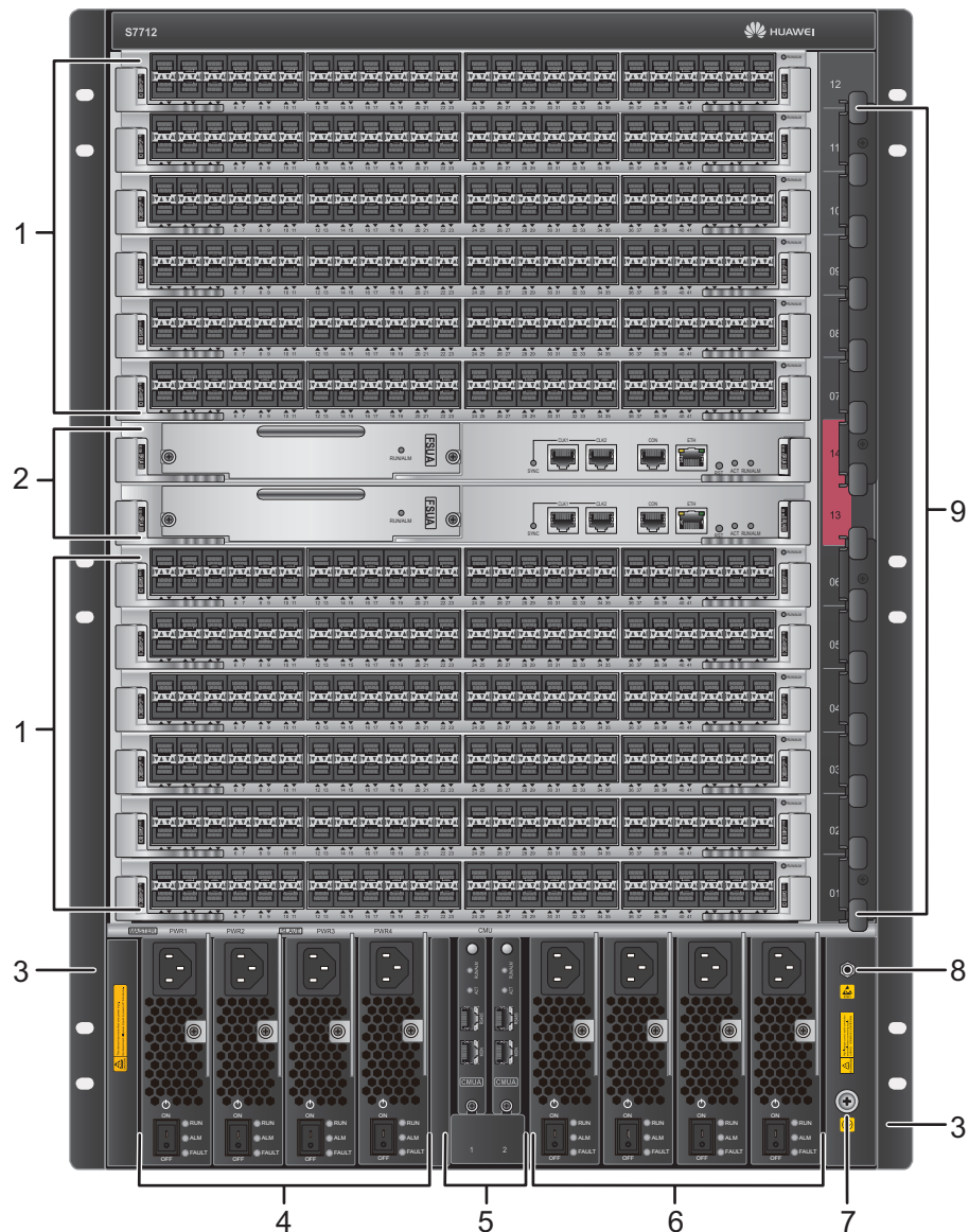
Figure 4-9 S7712 chassis structure (front view)
