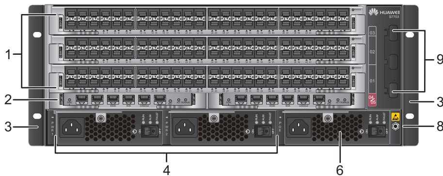
Figure 4-7 S7703 chassis structure (front view)
