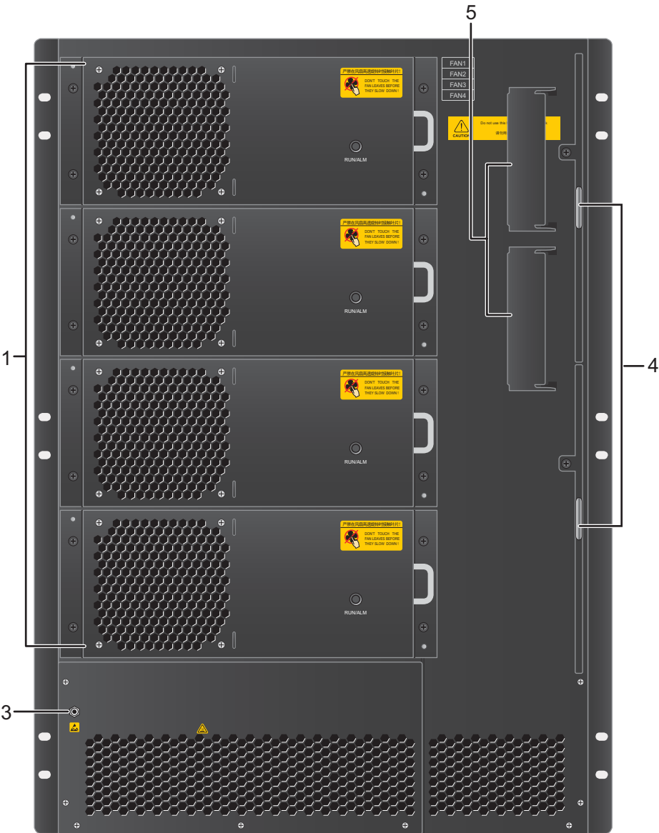
Figure 4-12 S7712 chassis structure (rear view)
