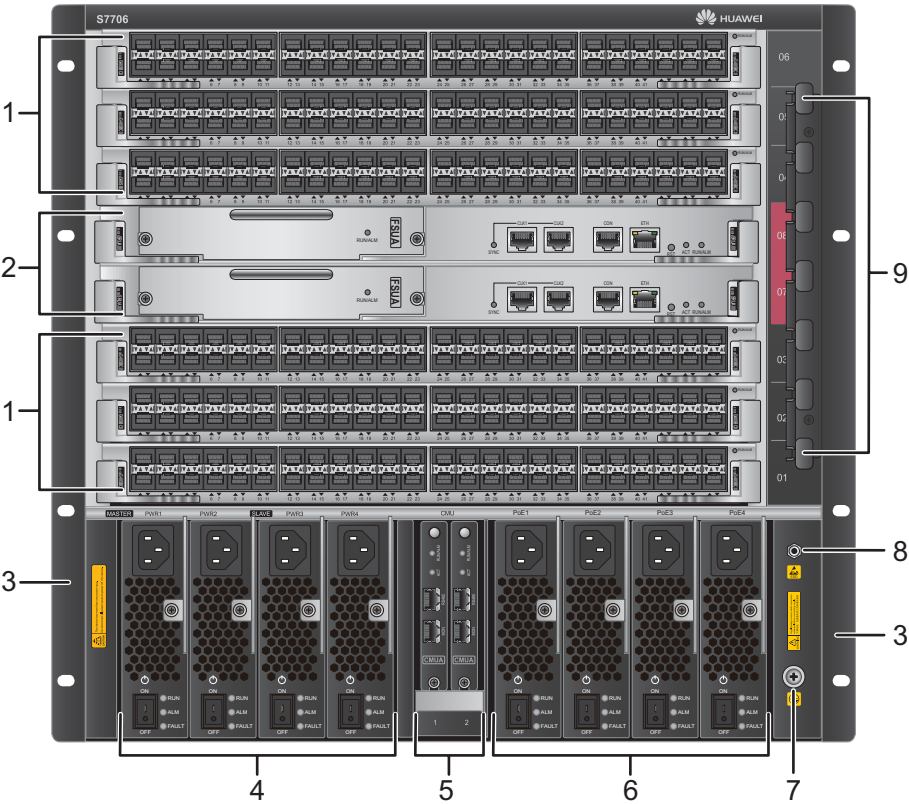
Figure 4-8 S7706 chassis structure (front view)
