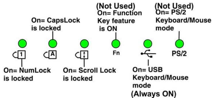
Figure 14- Keyboard LED Indications
